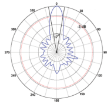
Vertical Beamwidth
