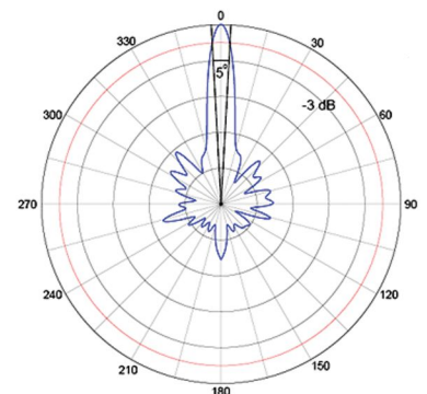
Vertical Beamwidth
