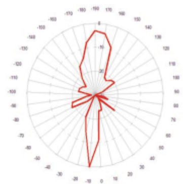
Vertical Beamwidth
