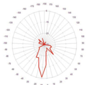
Vertical Beamwidth
